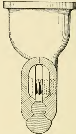
Fig. 188. Section Through Clamp for a "Figure 8" Wire
